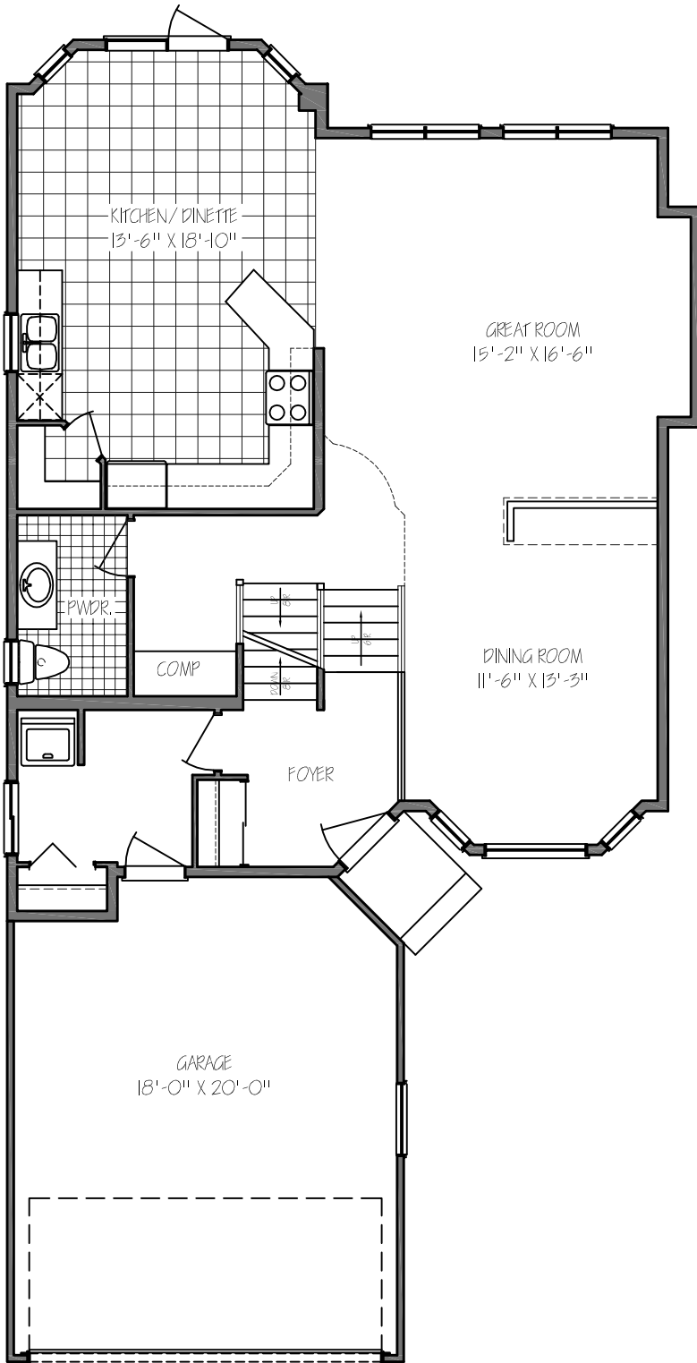
MAIN FLOOR PLAN 1024 Sq. Ft.
